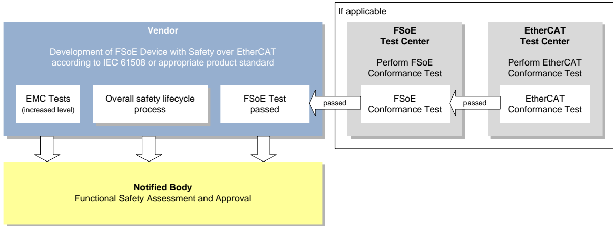
Figure 51: FSoE device assessment and approval
