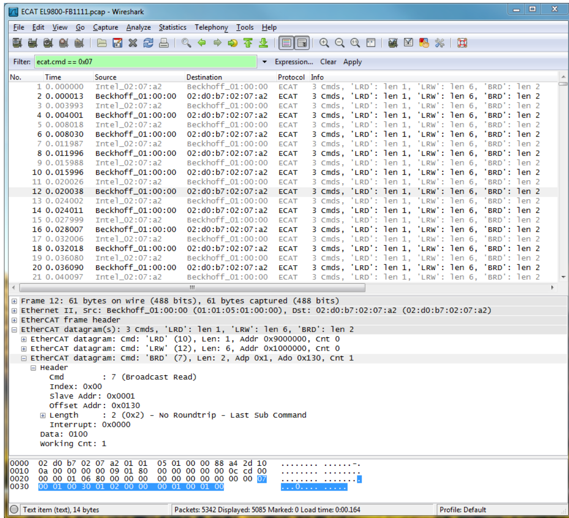
Figure 23: Wireshark Screenshot
