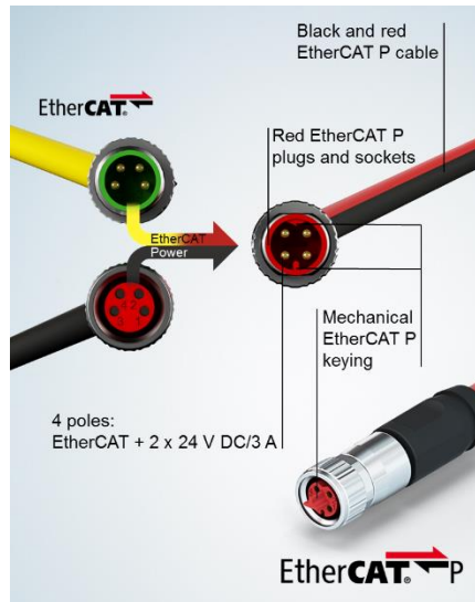
Figure 33: M8 P-coded connector and cable
