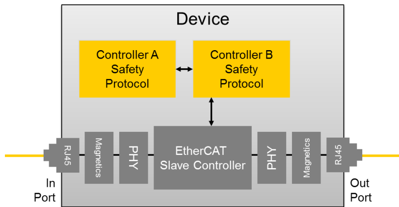
Figure 49: Hardware architecture
