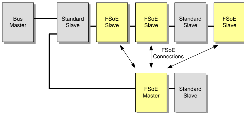
Figure 46: FSoE system architecture
