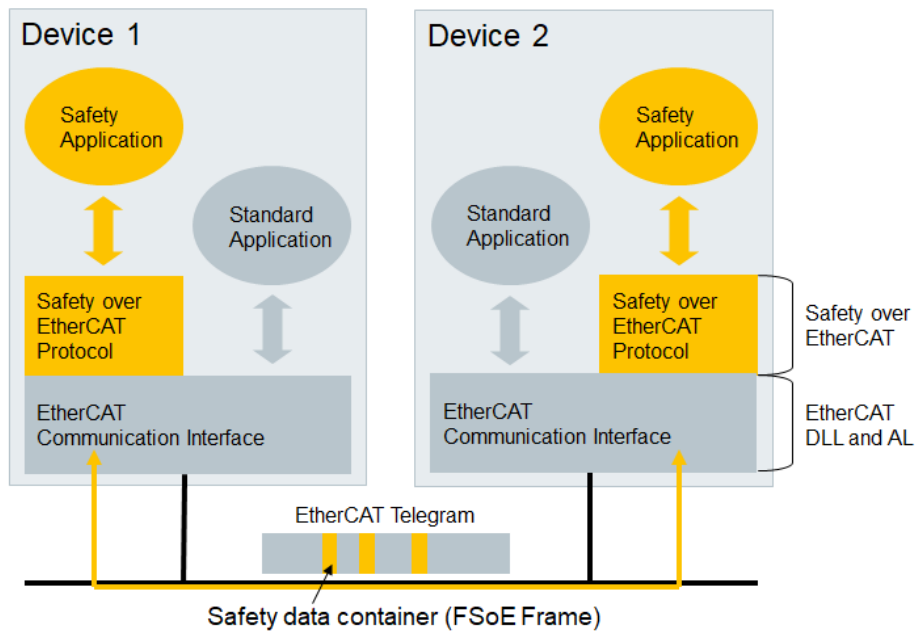
Figure 50: Software architecture
