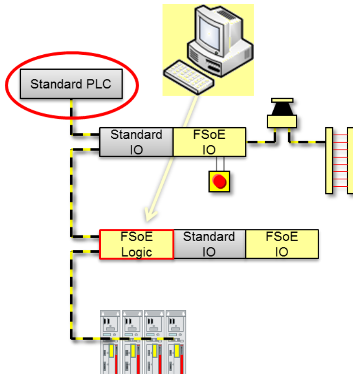
Figure 47: Decentralized safety logic approach with standard PLC
