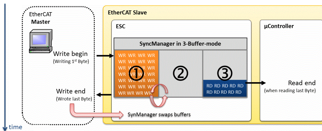
Figure 9: SyncManager 3-Buffer-Mode
