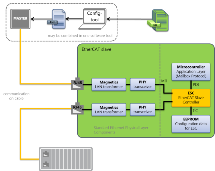
Figure 37: A typical EtherCAT device structure
